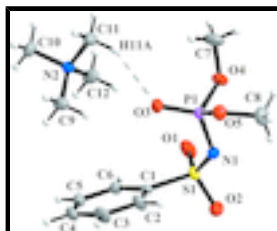
Fig. 1. The asymmetric unit of dimethyl(phenylsulfonyl)amidophosphato-tetramethylammonium. Displacement ellipsoids are drawn at the 20% probability level; hydrogen atoms are drawn as spheres of arbitrary radius.
