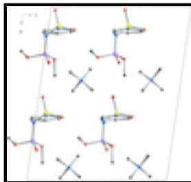
Fig. 2. Projection of the structure \{\text{N}(\text{CH}_3)_4\}^+[\text{C}_6\text{H}_5\text{SO}_2\text{NP}(\text{O})(\text{OCH}_3)_2]^- on the ac plane.
